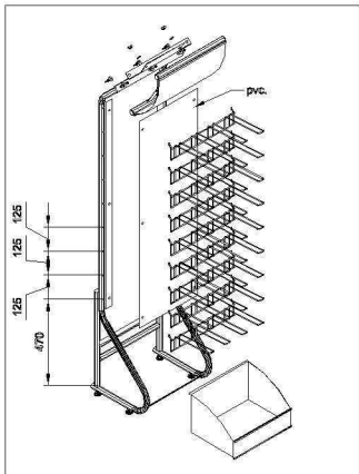
ASSEMBLY DRAWING
