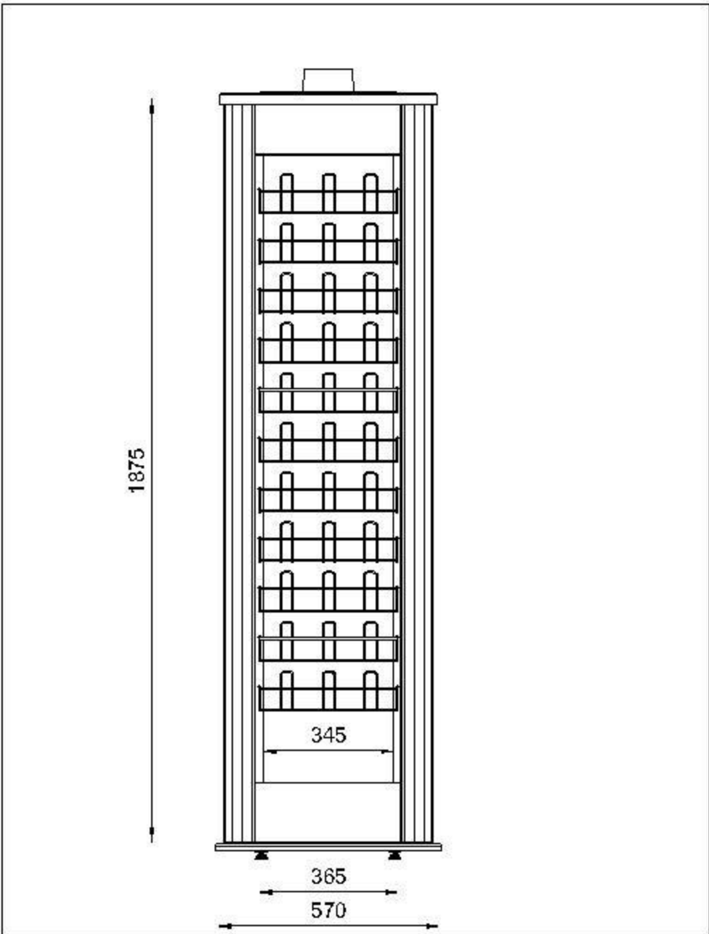
FRONT VIEW
