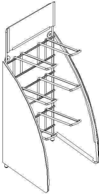
ISOMETRIC DRAWING
